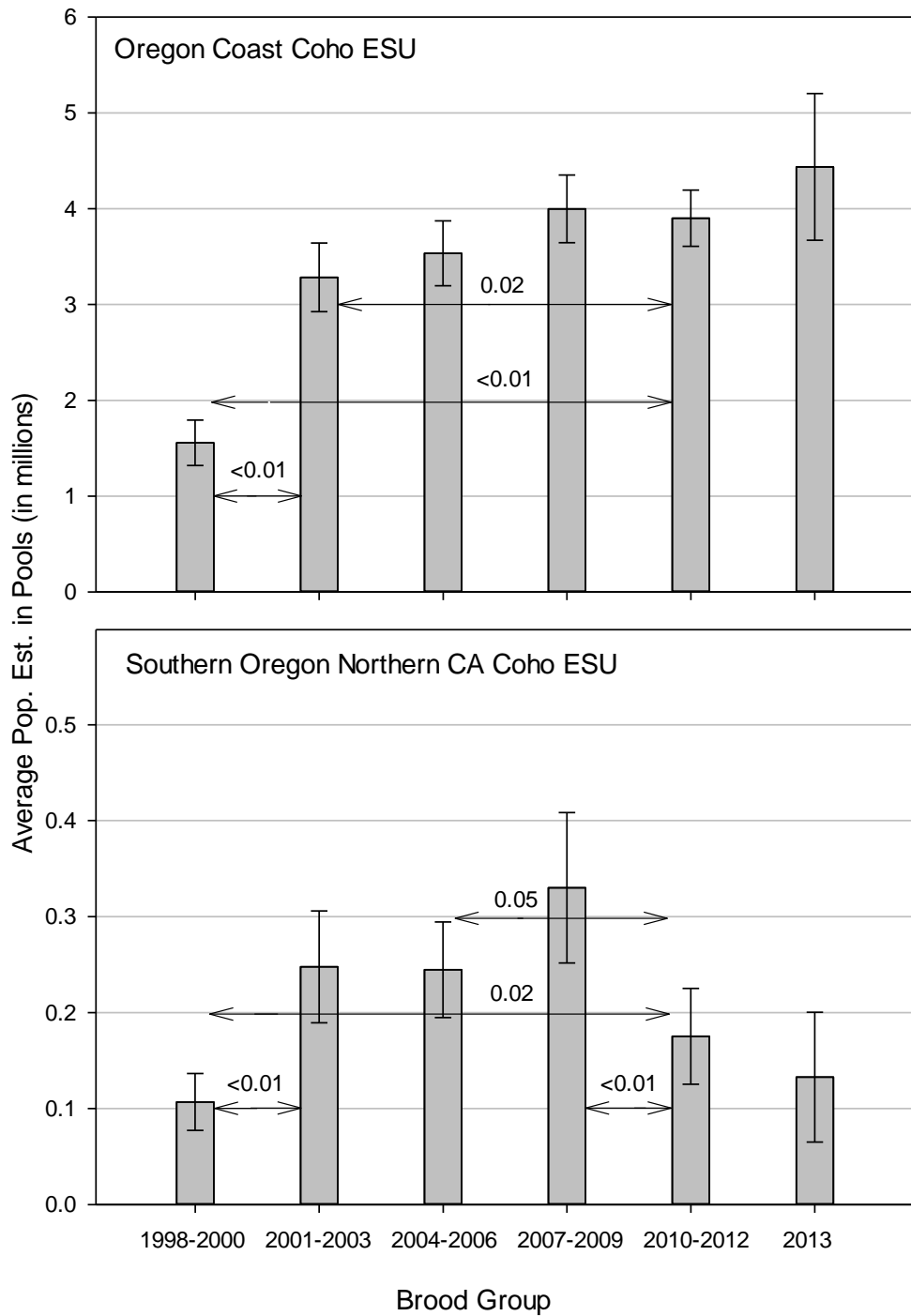
Trends in average pool population estimates of coho by brood group in the Oregon Coast Coho ESU (top panel) and Southern Oregon Northern California Coho ESU (bottom panel). Note the difference in Y-axis scale between the two panels. Gray bars show the population estimate (with 95%CI) for the brood group, p values for comparisons among brood groups are given above each vertical arrow where differences are significant.
