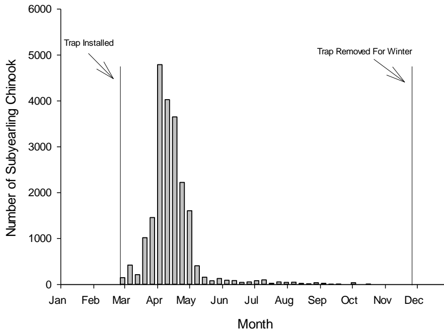
Figure 20. Weekly catch of subyearling spring Chinook salmon captured in the South Fork McKenzie River trap above Cougar Reservoir, 2016.
