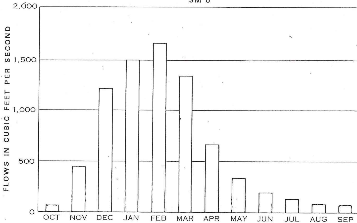
Figure 2. Mean monthly flow in the Yaquina River at river mile 0 (State Water Resource Board 1974).
