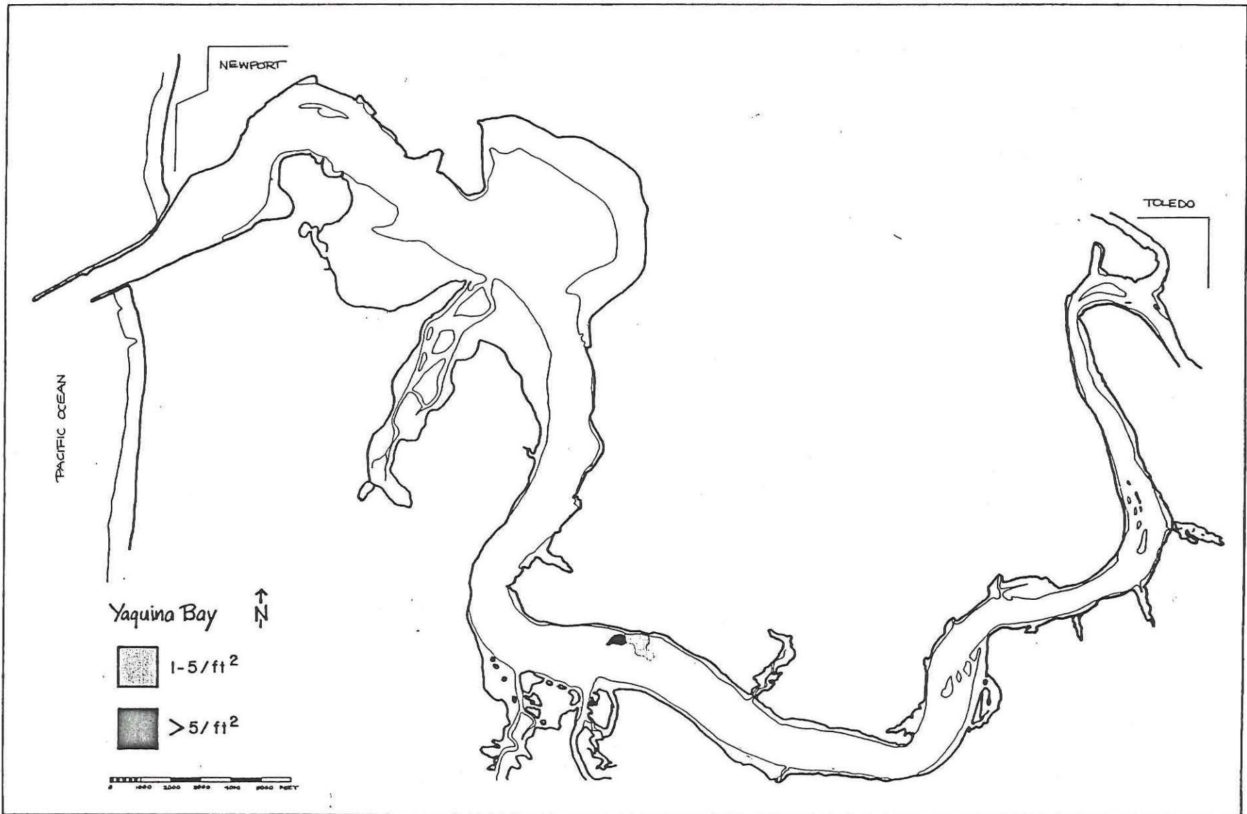
Figure 15. Distribution of native oysters in Yaquina Bay (Hancock et al. 1979)
