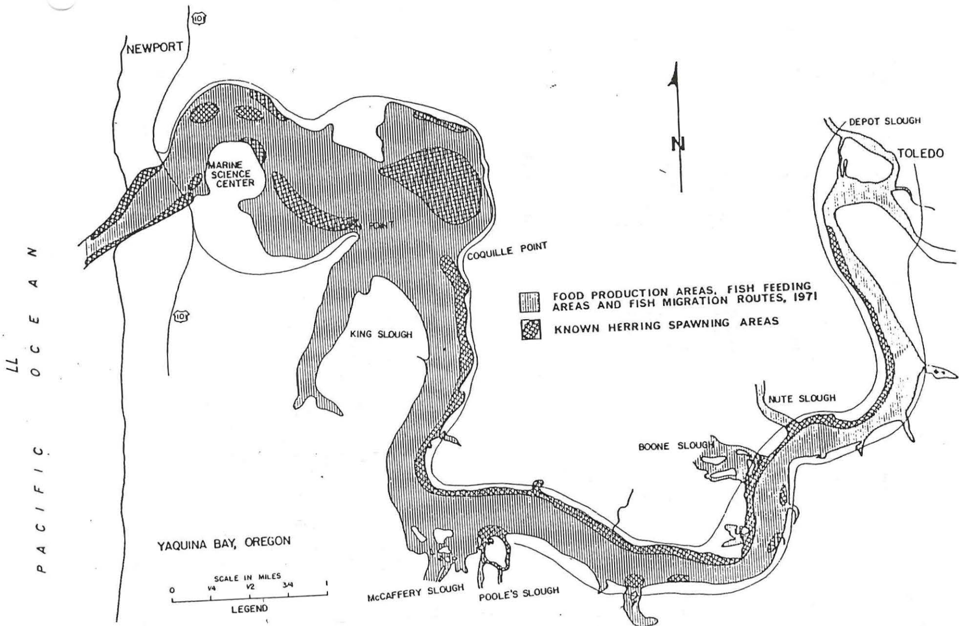
Figure 8. Areas of Yaquina Bay used for spawning by Pacific herring (Gaumer et al. 1974).
