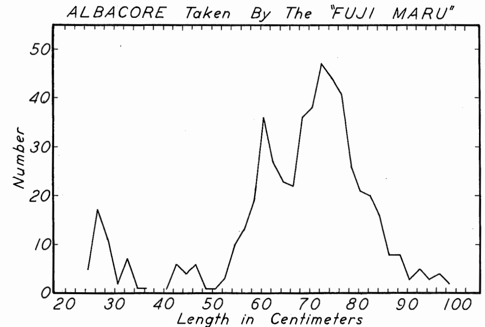
Fig. 19. Length-frequency curve for albacore taken by the "Fuji Maru." Data from Figure 7 of Aikawa and Katô, 1938.
