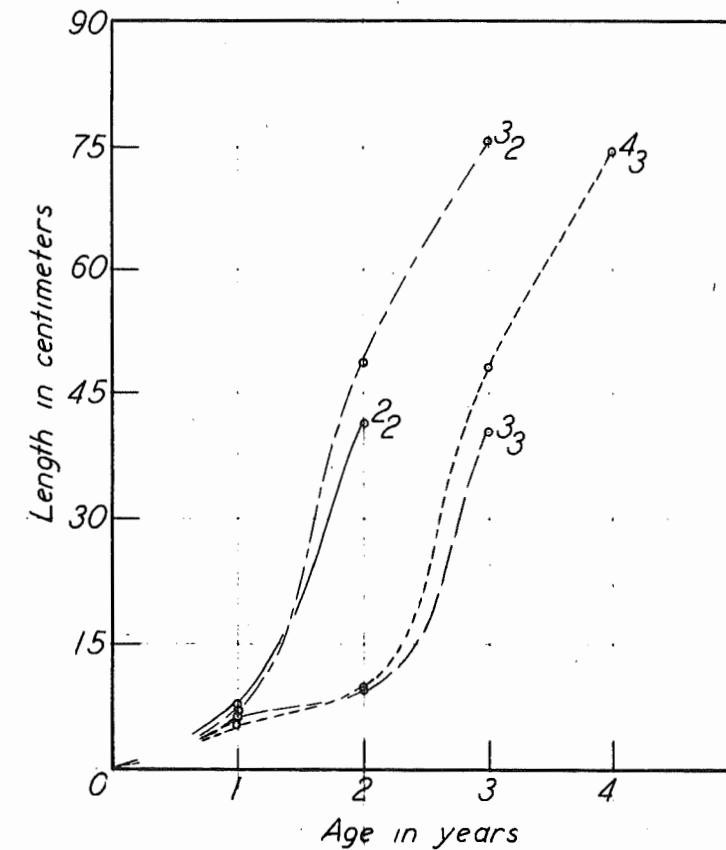
Fig. 20. Silvers: growth curves for all age categories.
