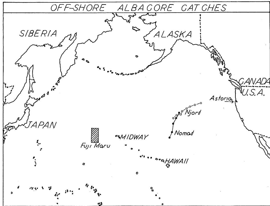
Fig. 18. Chart showing location of albacore catches in mid-Pacific. The rectangle west of Midway Island marks the position of the catches made by the "Fuji Maru" (Aikawa and Katô, 1938). The solid circles between the Hawaiian Islands and the American coast show the course over which albacore were landed aboard the "Nomad," and the open circles the course over which albacore were landed aboard the "Njord." The position given at the southern end of the "Nomad's" course is that of the initial albacore catch, and the position at the northern end of the course of the "Njord" is that of the last albacore catch of that yacht.
