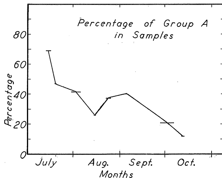
Fig. 12. Percentages of albacore of group A in the samples taken from the Oregon catch for July 30—Oct. 14, 1940.
