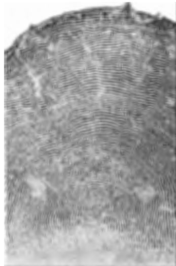
Fig. 5. Chum: scale from a five-year-old male, 82 centimeters long, taken in the lower Columbia River on October 13, 1914.
