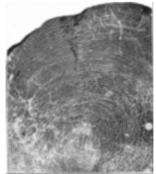
Fig. 18. Silver: scale from a four-year-old female that had gone to sea in its third year ( 4_s ), 74 centimeters long, taken in the lower Columbia River on November 16, 1914.
