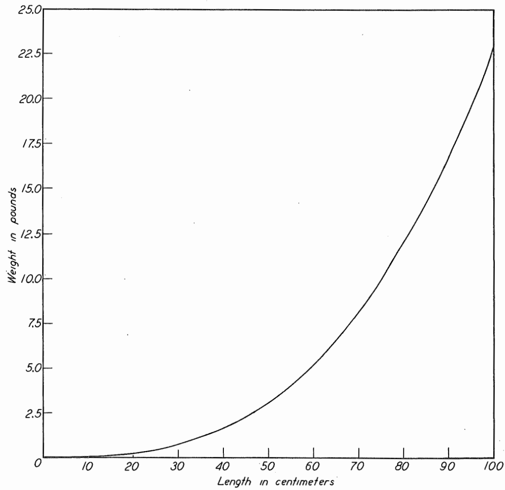
Fig. 21. Silvers: length-weight curve based on 605 Columbia River specimens, 37-92 centimeters in length.
