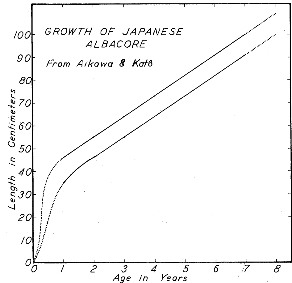
Fig. 17. Growth curve of Japanese albacore according to the data of Aikawa and Katô, 1938.
