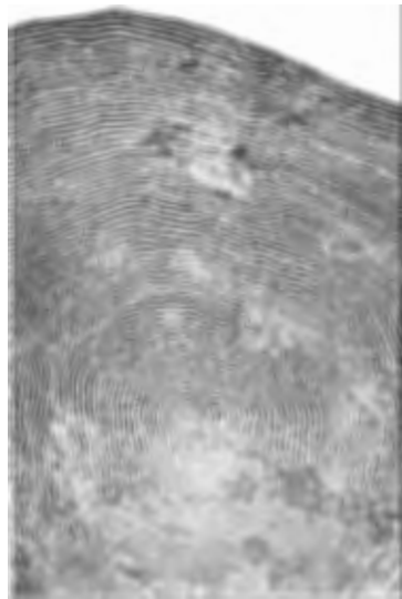
Fig. 4. Chum: scale from a four-year-old female, 77 centimeters long, taken in the lower Columbia River on October 22, 1914.
