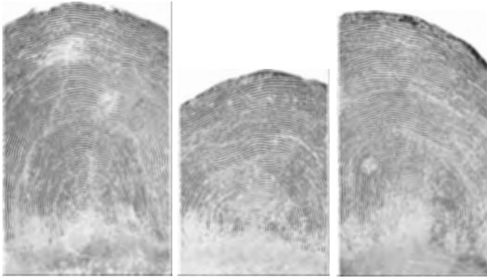
Fig. 1. Chum: scale from a three-year-old male, 74 centimeters long, taken in the lower Columbia River on November 20, 1914.
