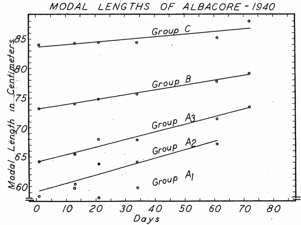
Fig. 11. Modal lengths of Astoria albacore, July 30-Oct. 14, 1940. The graduating straight lines were fitted by least squares.
