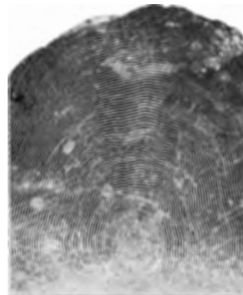
Fig. 17. Silver: scale from a four-year-old male that had gone to sea in its third year ( 4_s ), 79 centimeters long, taken in the lower Columbia River on October 22, 1914.
