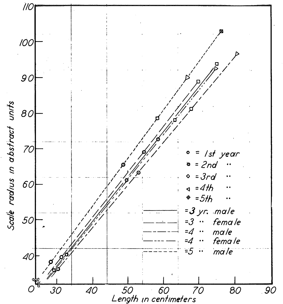
Fig. 7. Chums: relation of scale radius to fish length in Columbia River chums, grouped by sex and age.
