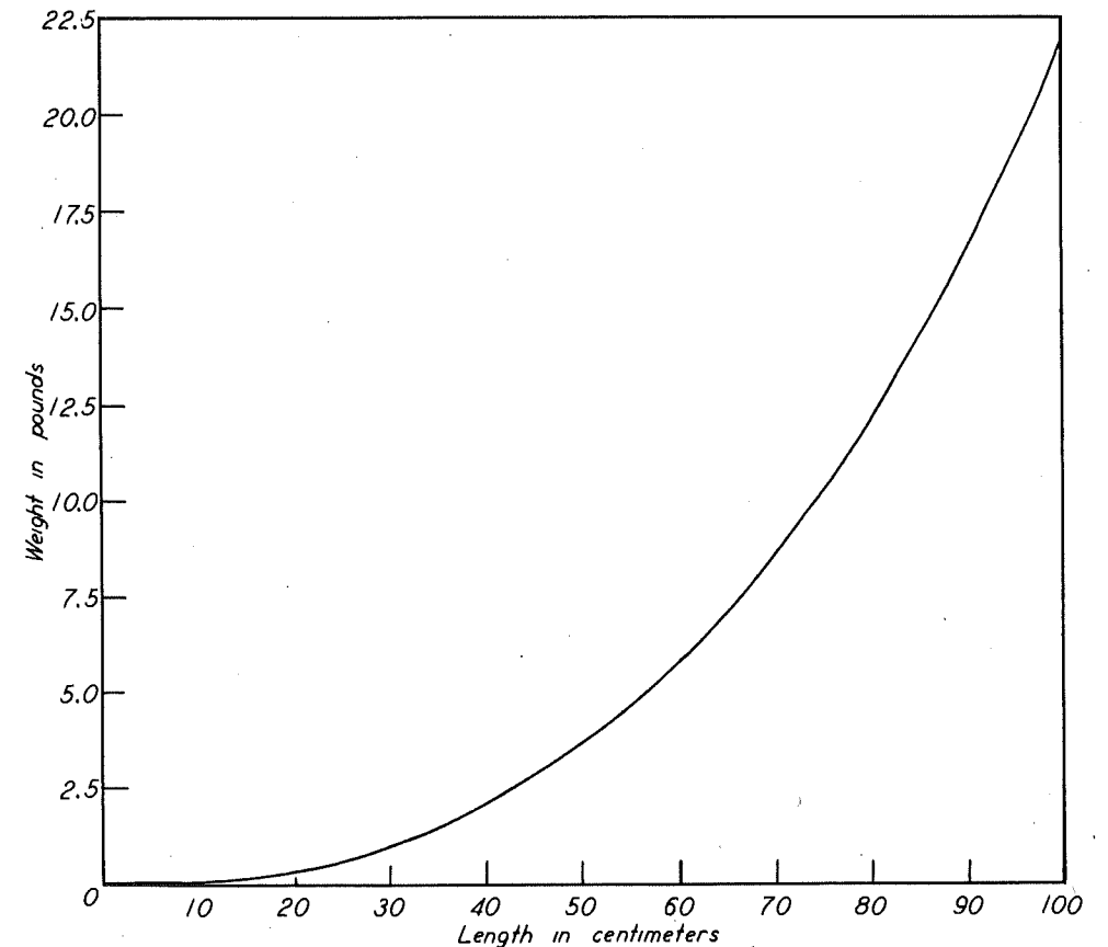
Fig. 9. Chums: length-weight curve based upon 375 Columbia River specimens, 60-92 centimeters in length.
