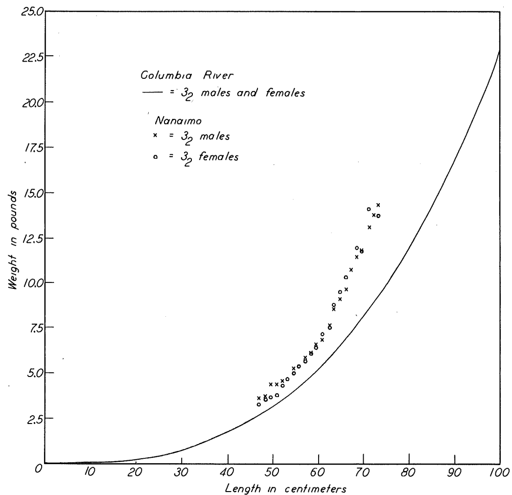
Fig. 23. Silvers: comparison of the length-weight relationship in samples from the Columbia River and Nanaimo.
