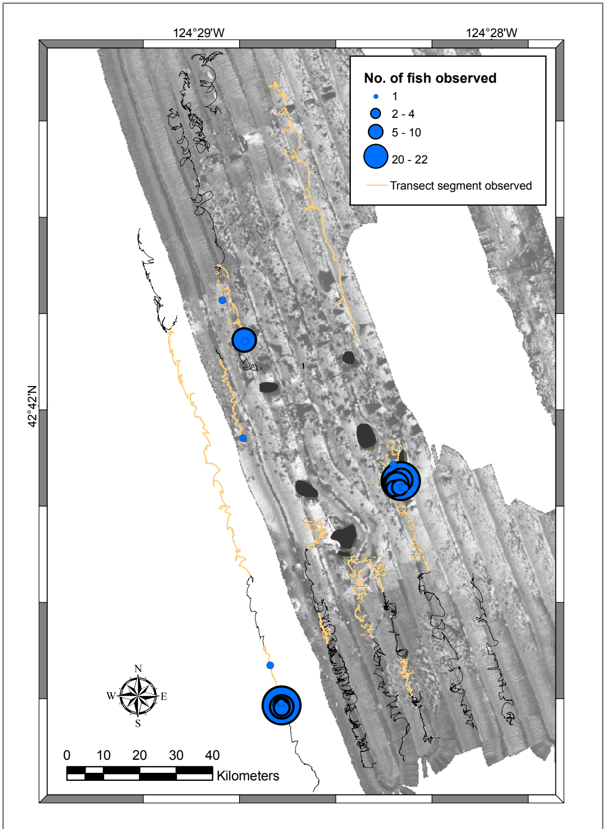
Figure 10b. Spatial distribution of blue rockfish along ROV video transects and overlaid on sidescan sonar imagery.
