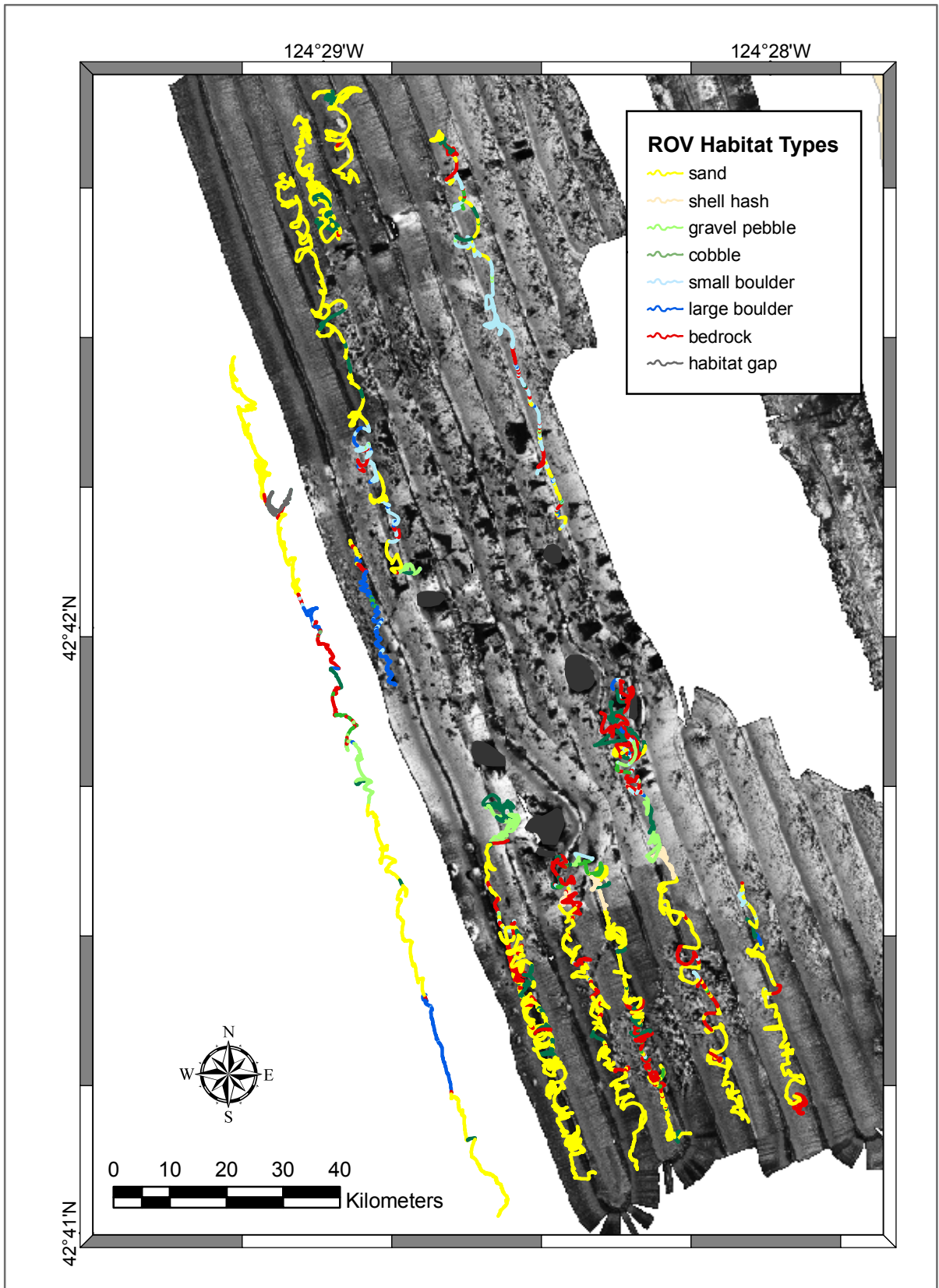
Figure 8a. Map of color-coded ROV habitat types overlaid on sidescan sonar imagery.
