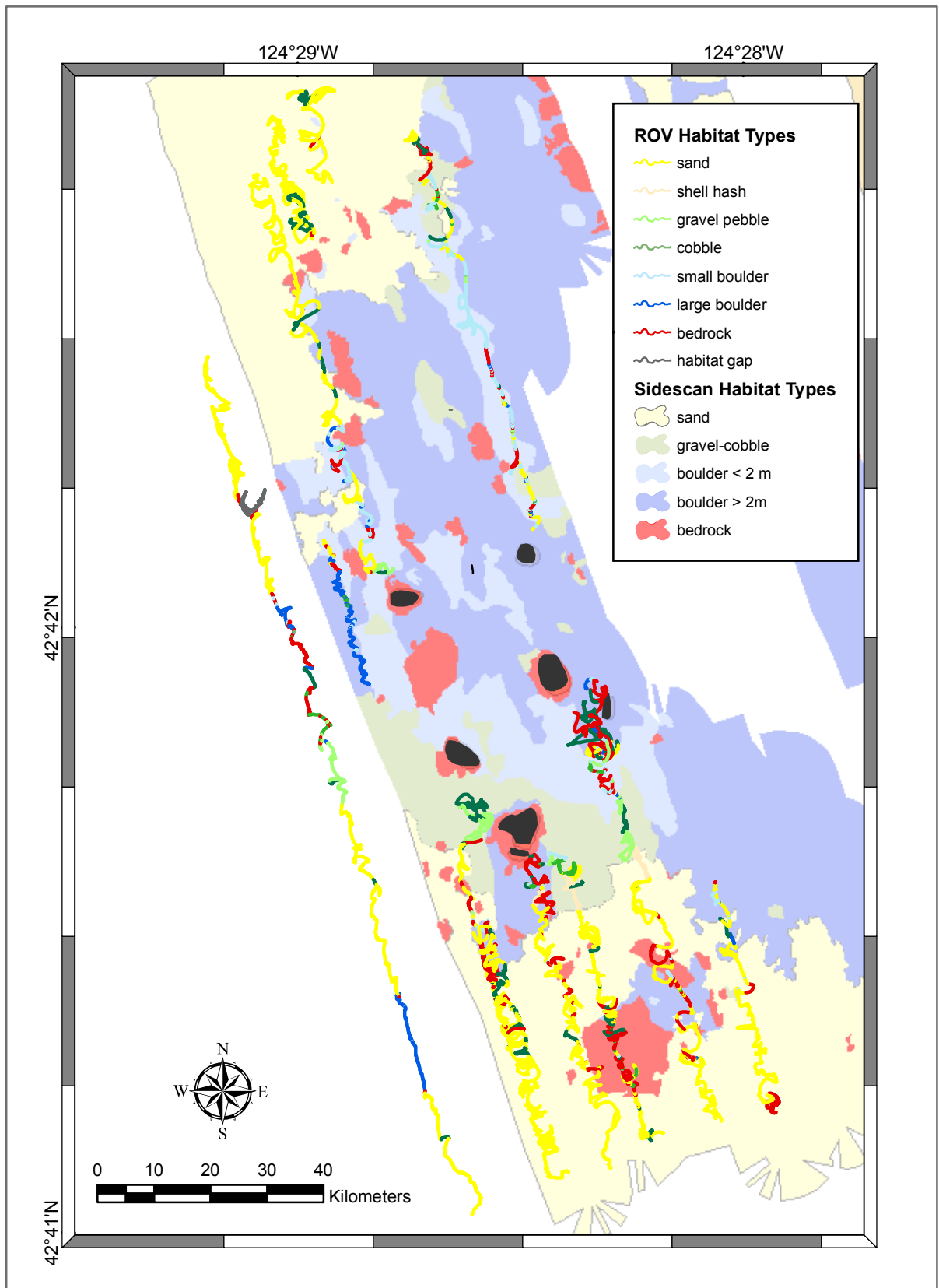
Figure 8b. Map of color-coded ROV habitat types overlaid on polygons of habitat types interpreted from sidescan sonar imagery.
