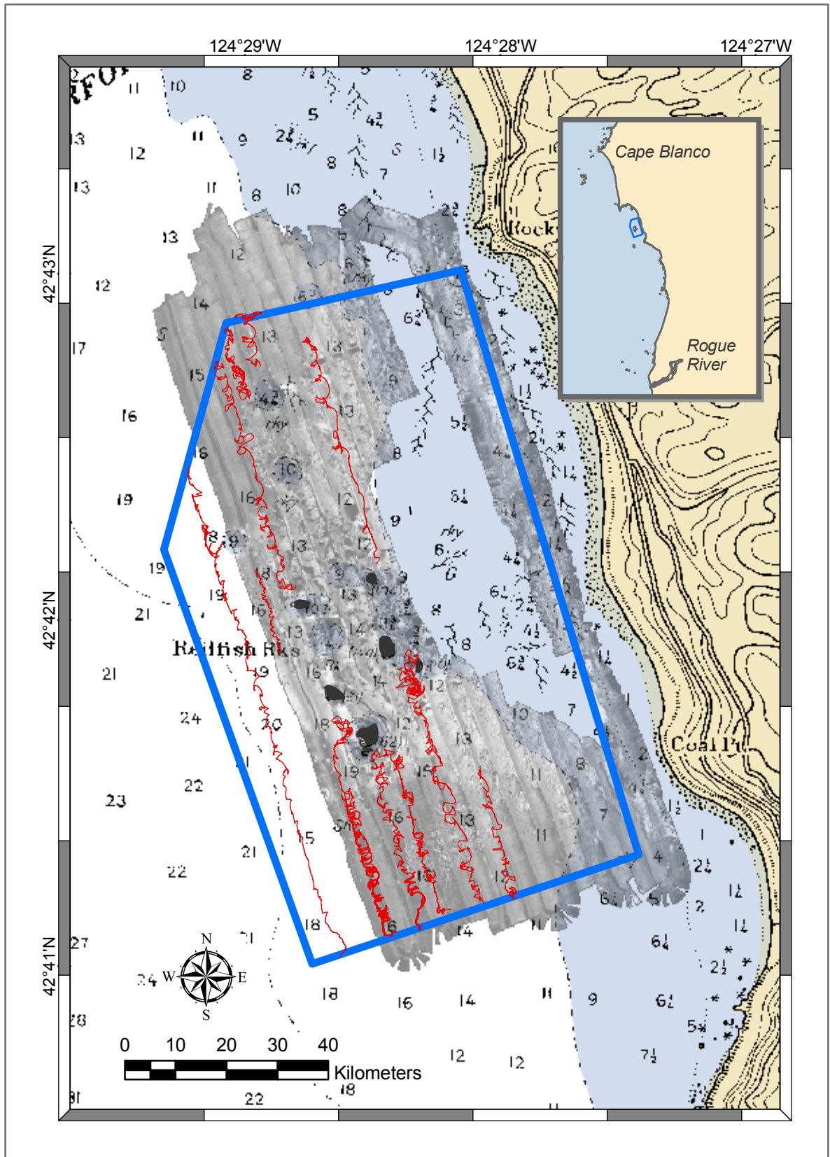
Figure 7. Map of surveyed ROV transects overlaid on sidescan sonar imagery.
