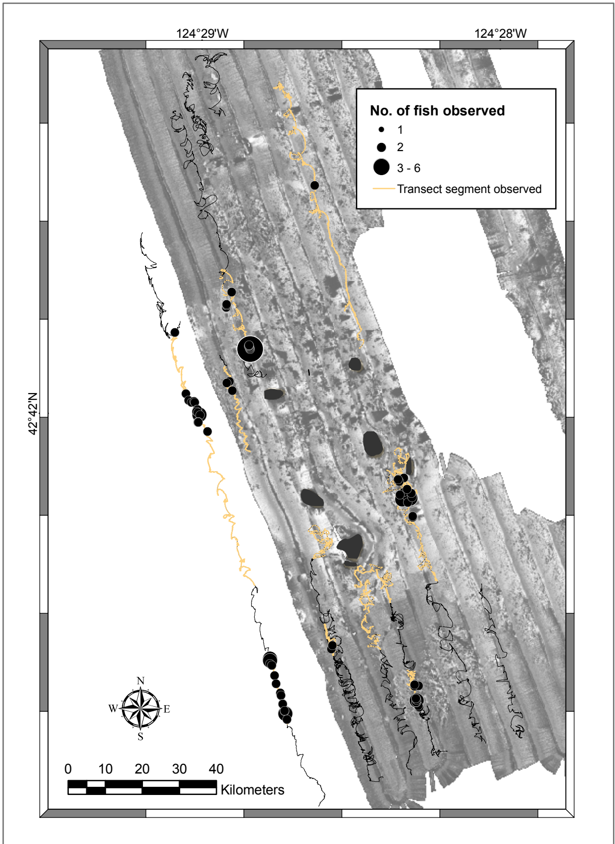
Figure 10a. Spatial distribution of black rockfish along ROV video transects and overlaid on sidescan sonar imagery.
