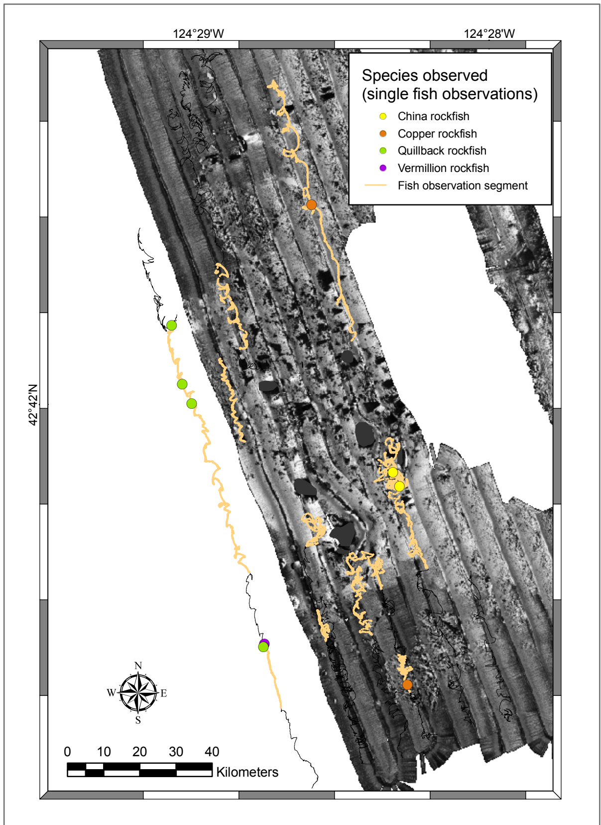
Figure 10d. Spatial distribution of demersal rockfishes (China, Copper, Quillback and Vermillion) along ROV video transects and overlaid on sidescan sonar imagery.
