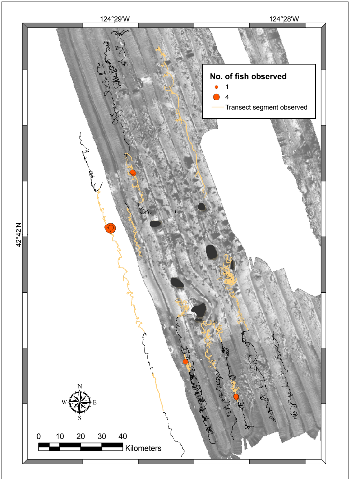
Figure 10c. Spatial distribution of canary rockfish along ROV video transects and overlaid on sidescan sonar imagery.
