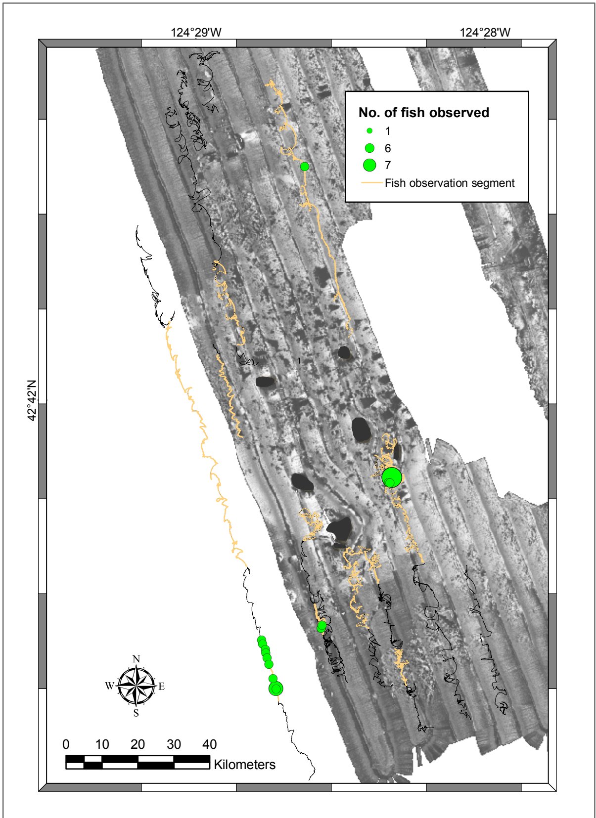
Figure 10e. Spatial distribution of unidentified rockfish along ROV video transects, overlaid on sidescan sonar imagery.
