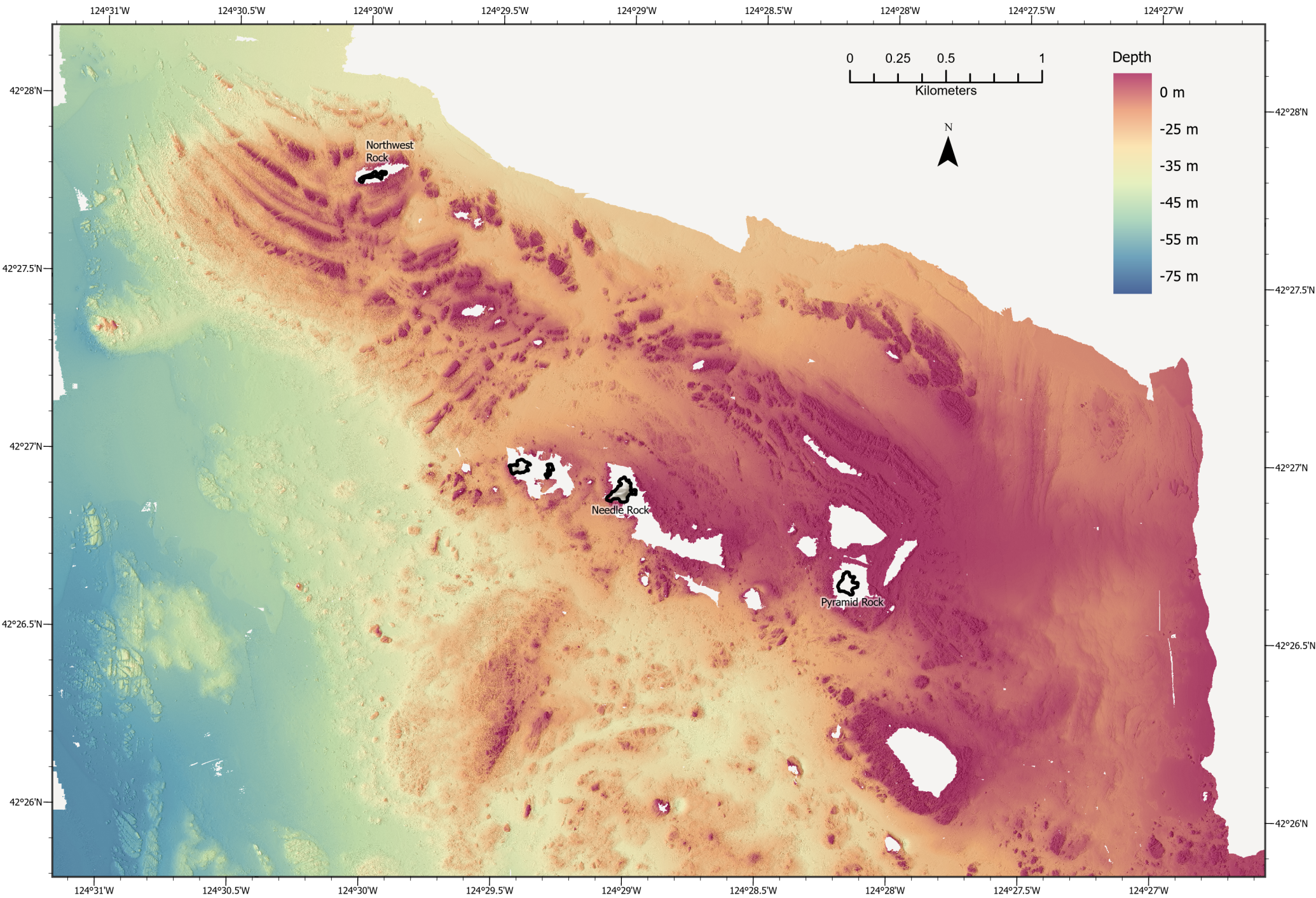
Northern section of ODFW bathymetry survey data at Rogue River Reef. Areas in white are data gaps, and may represent features that presented hazards to navigation during the survey (islands, submerged rocks, mounding waves, or kelp at the surface), or simply gaps between survey vessel transits. Map not intended for navigation.
