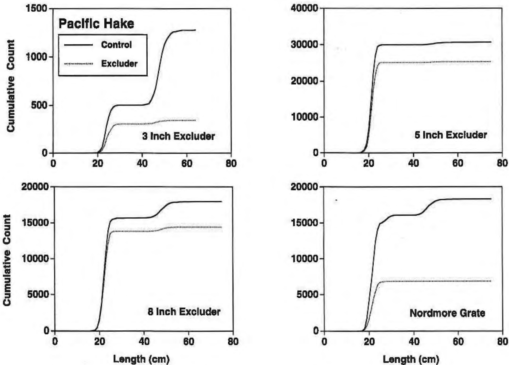
Figure 9. Cumulative length frequency distribution (cm) of Pacific hake retained by the experimental and control nets during tests of four fish excluder devices.
