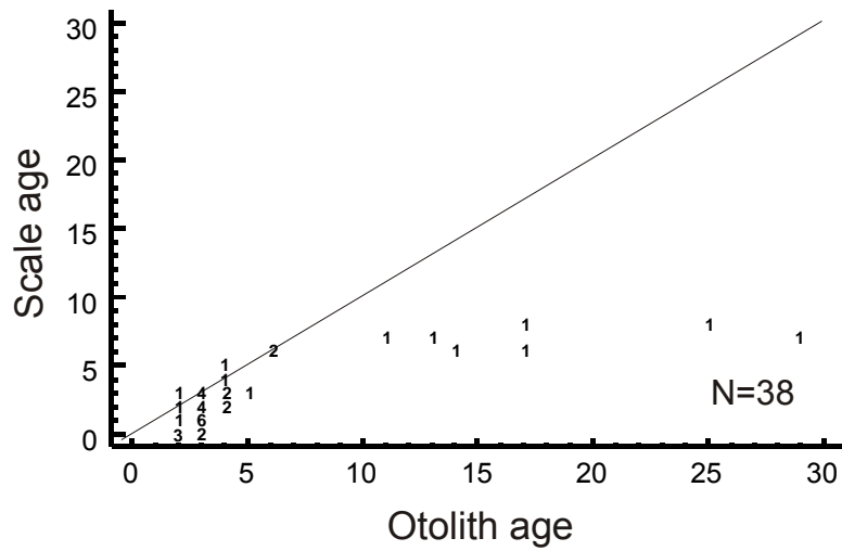
Figure 10. Age bias plots comparing ages from lapilli (otoliths) with other hard structures. Points that fall along the 45° line represent no ageing bias. Sample sizes varied between comparisons due to the inability to read all structures from all fish.
