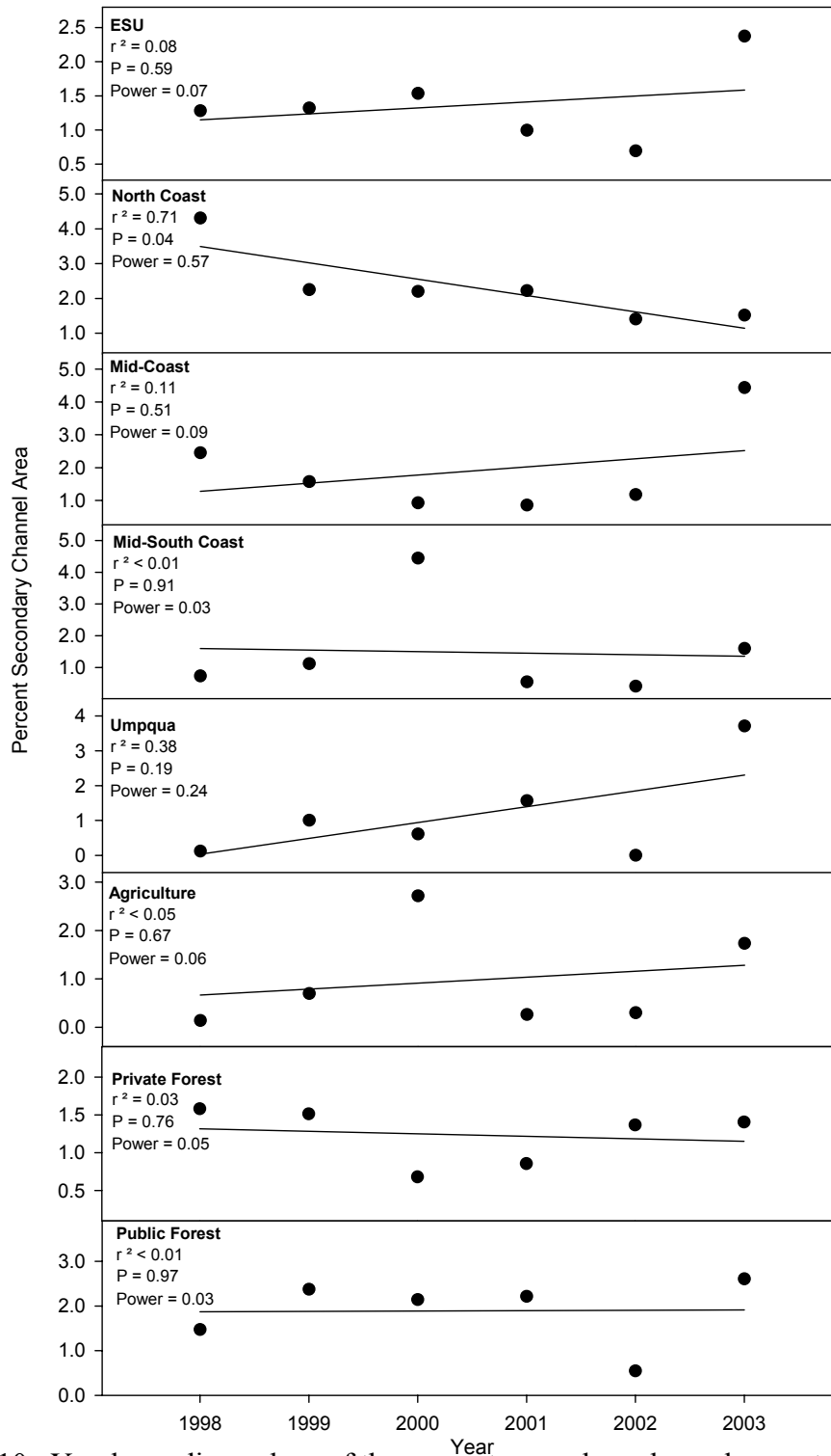
Figure 10. Yearly median values of the percent secondary channel area at the ESU, monitoring area, and landuse scale.
