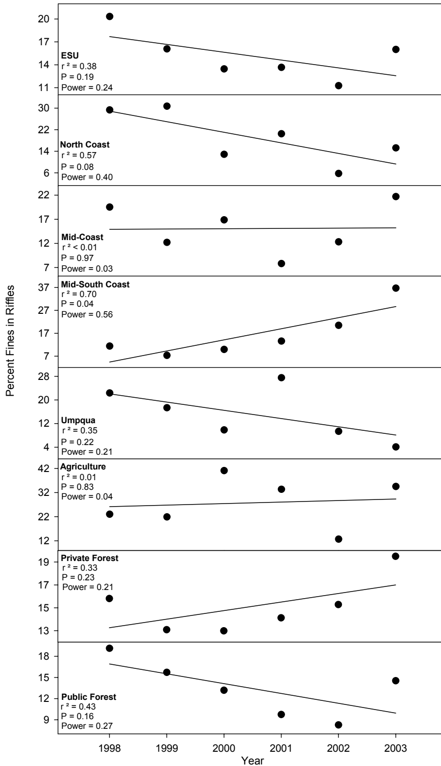
Figure 22. Yearly median values of percent fines in riffles at the ESU, monitoring area, and landuse scale.
