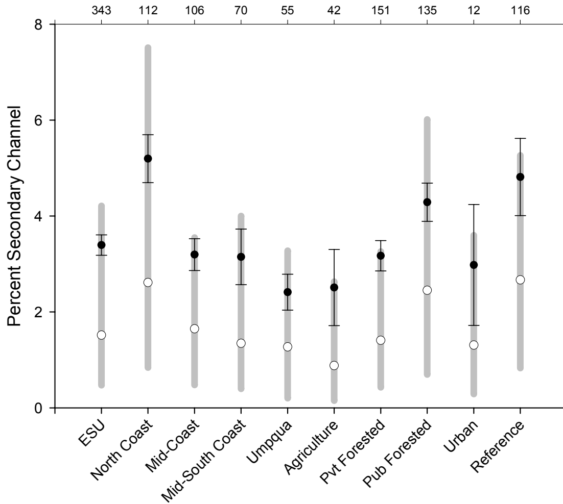
Figure 6. The percentage of secondary channel at reference sites and for random surveys conducted at the ESU, monitoring area, and landuse scales from 1998-2003.
