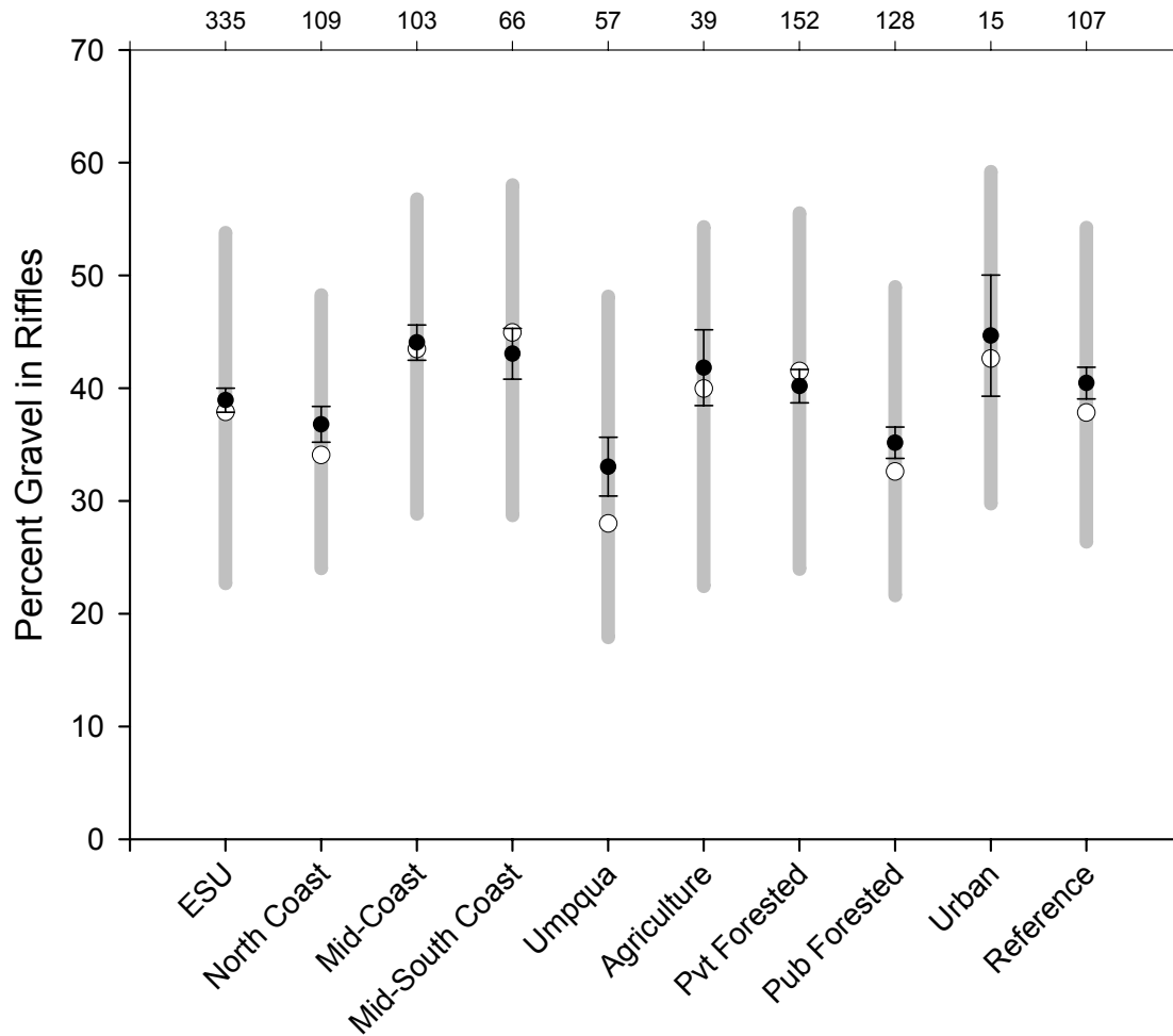
Figure 20. The percent of gravel in riffles at reference sites and for random surveys conducted at the ESU, monitoring area, and landuse scales from 1998-2003.
